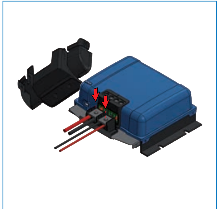
STEP 2: After mounting the MPPT to the wall, secure the cables.
