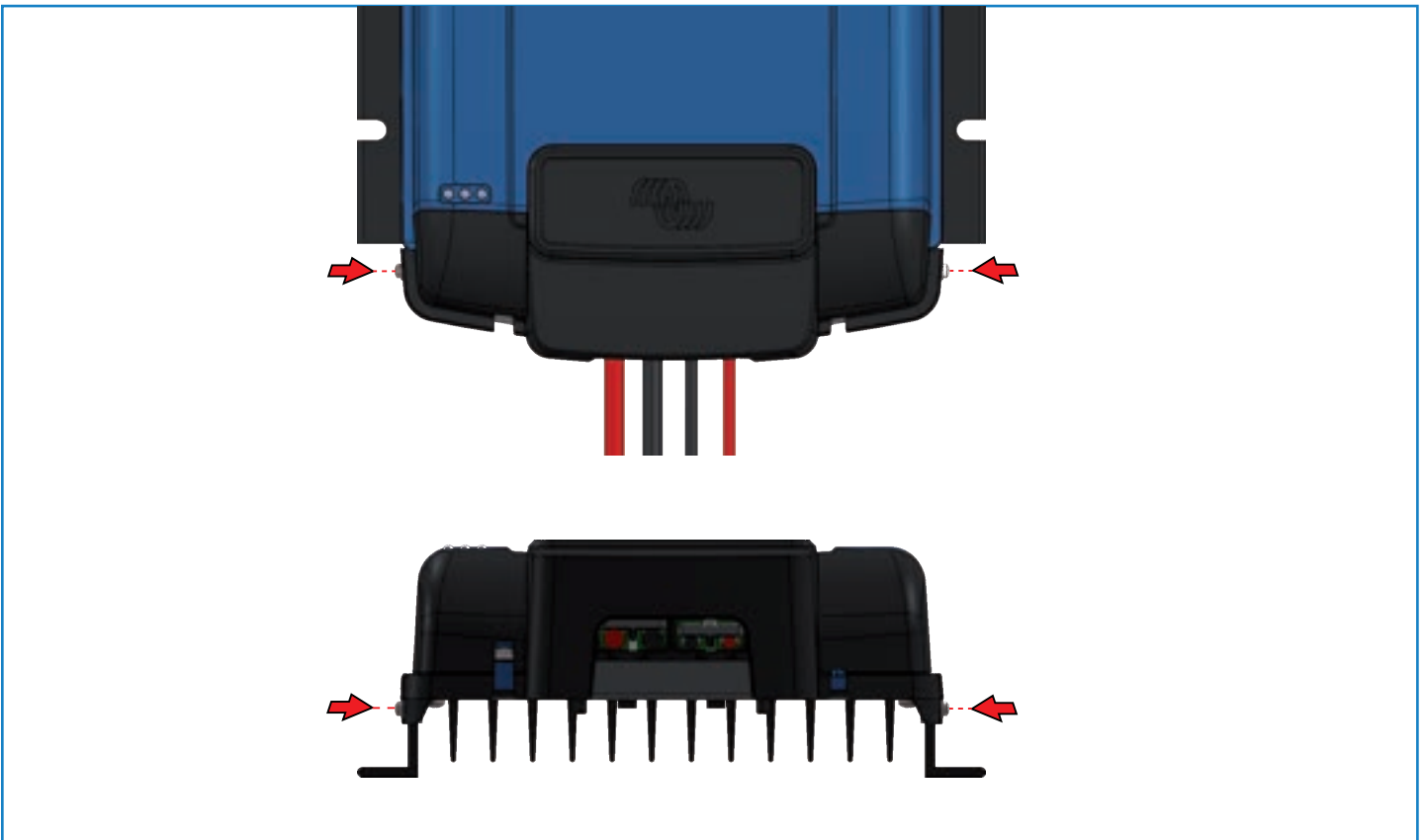
STEP 3: Place the WireBox cover and fasten with two screws.
